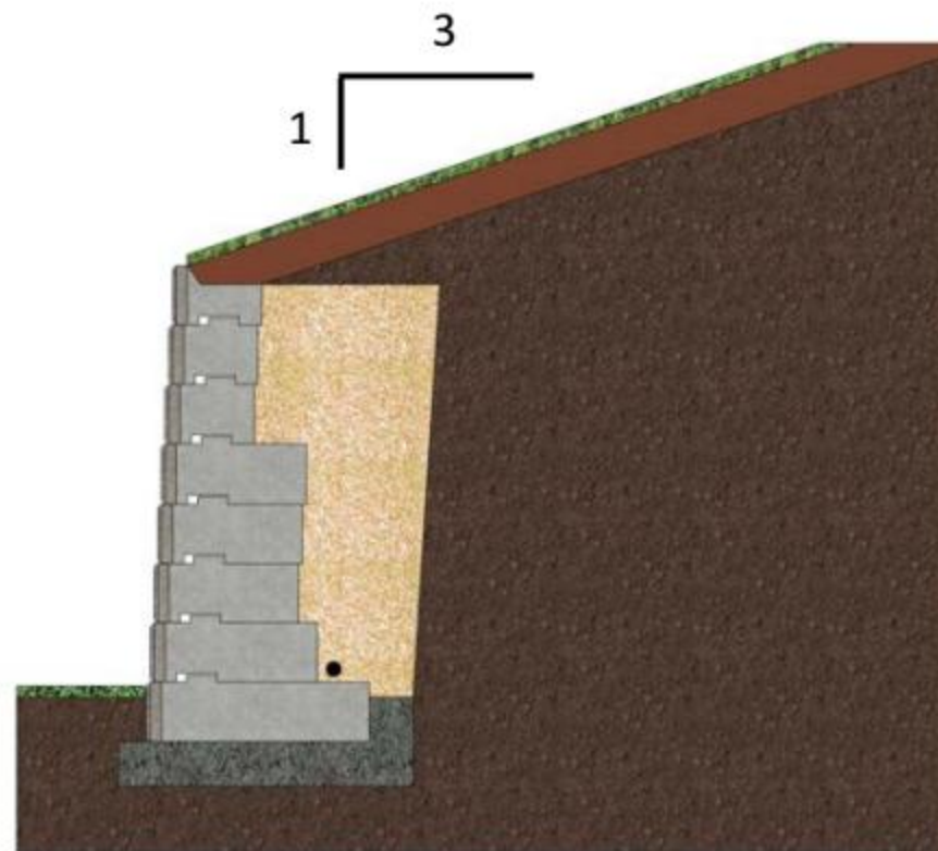
3H:1V Backslope—No Surcharge
