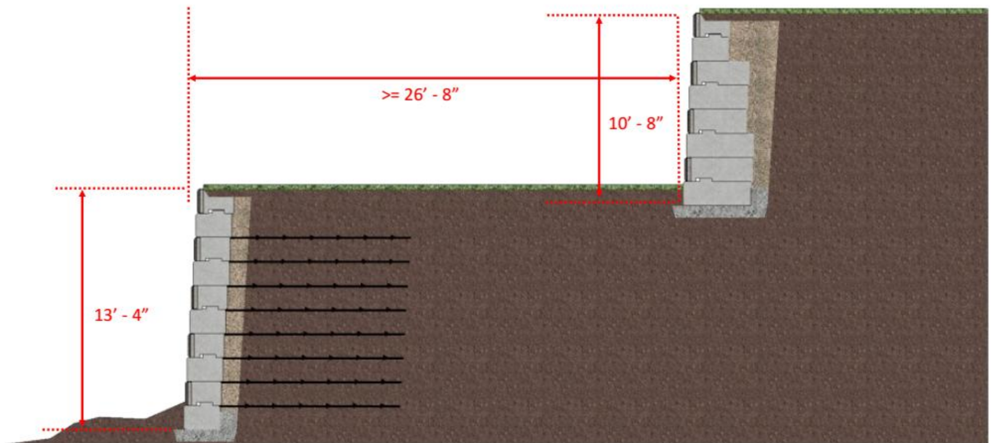
Terraced Wall Example
