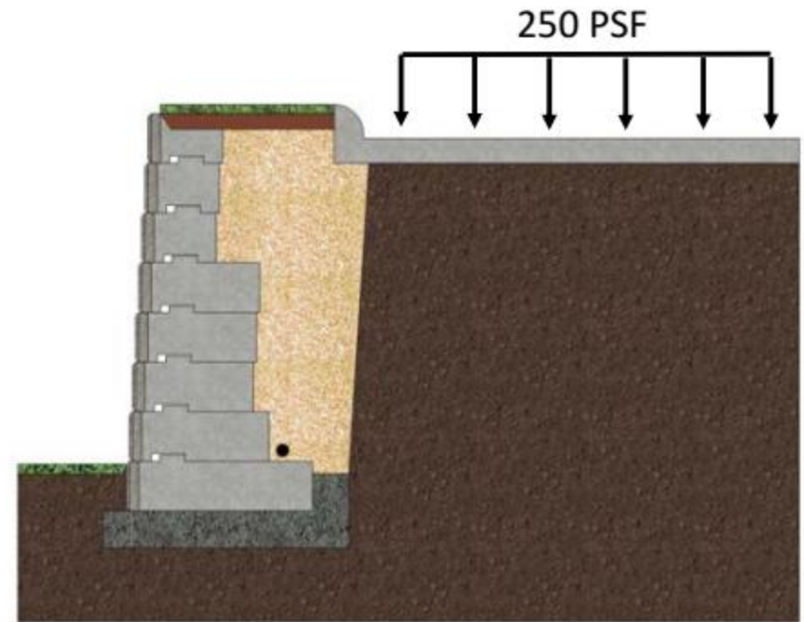
Level Backslope — 250 PSF Surcharge
