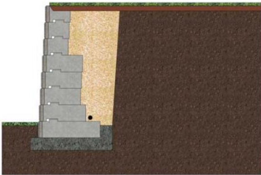
Level Backslope — No Surcharge
