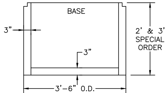
SECTION VIEW
