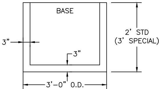
SECTION VIEW
