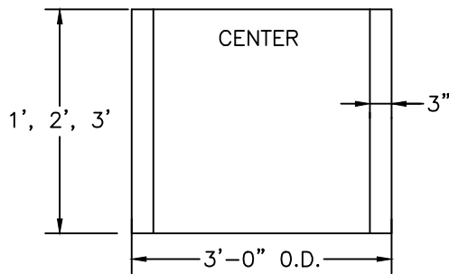
SECTION VIEW
