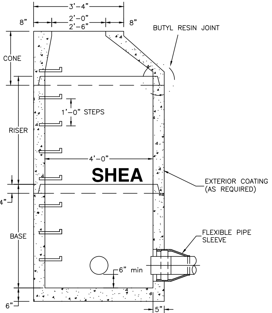
SECTION VIEW
