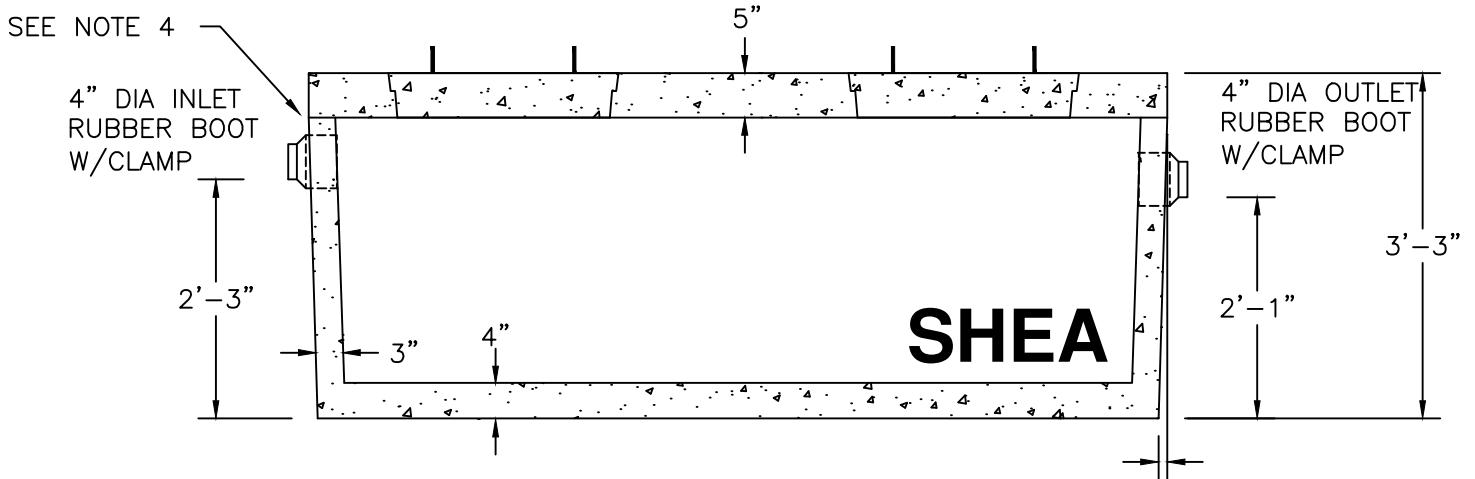
SECTION VIEW
