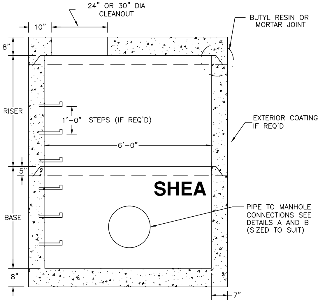
SECTION VIEW
