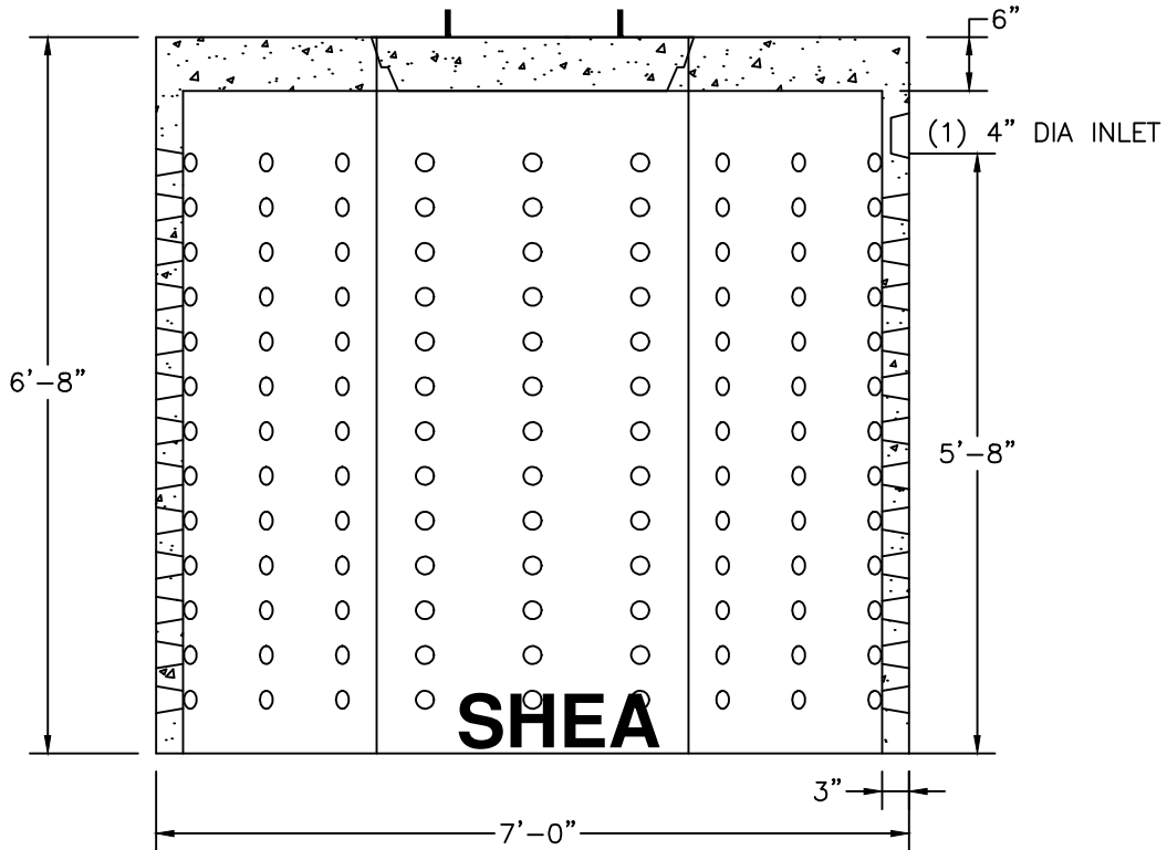
SECTION VIEW
