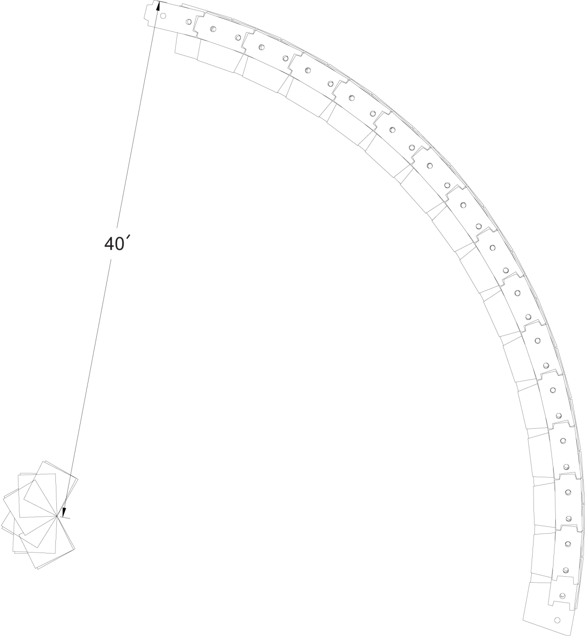
Shea Guardrail Block Minimum Turning Radius Outside Curve 40' Radius with 2" cut/removed from inside wing of Guardrail Block in field
