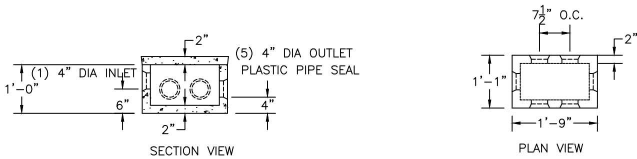
5 OUTLET STANDARD
