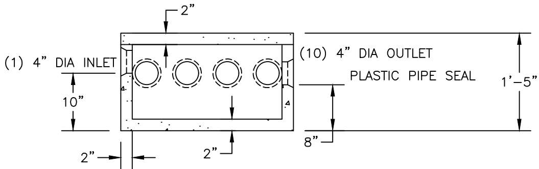
SECTION VIEW
