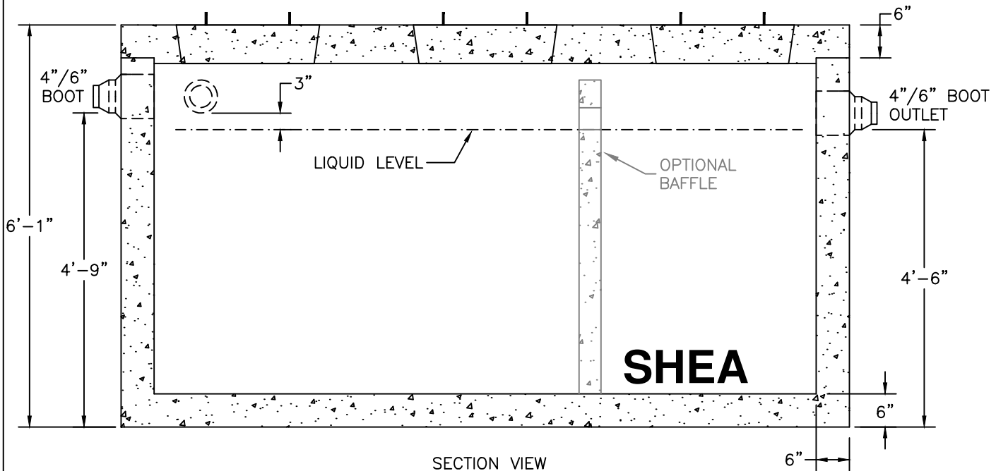
SECTION VIEW
