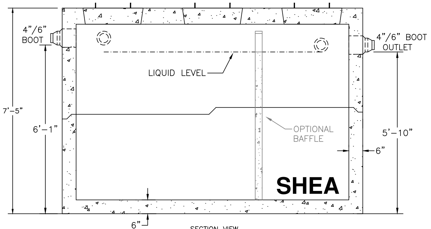
SECTION VIEW
