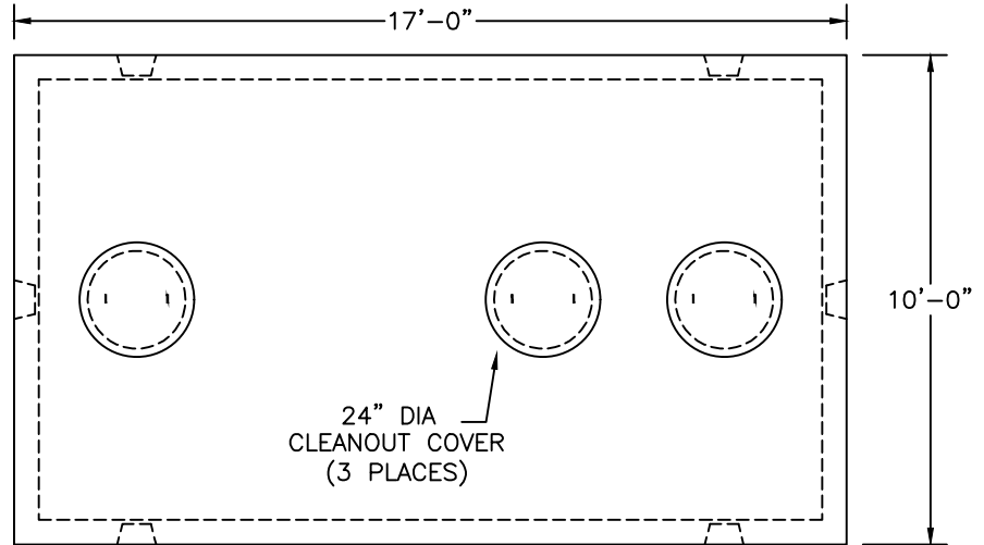
PLAN VIEW
