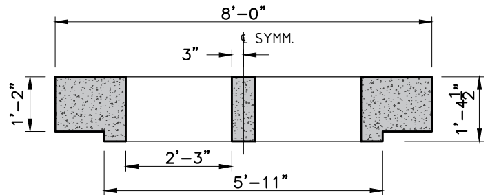
SECTION B-B
