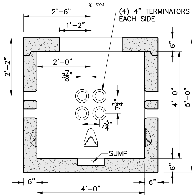
SECTION A-A CLOSED BOTTOM
