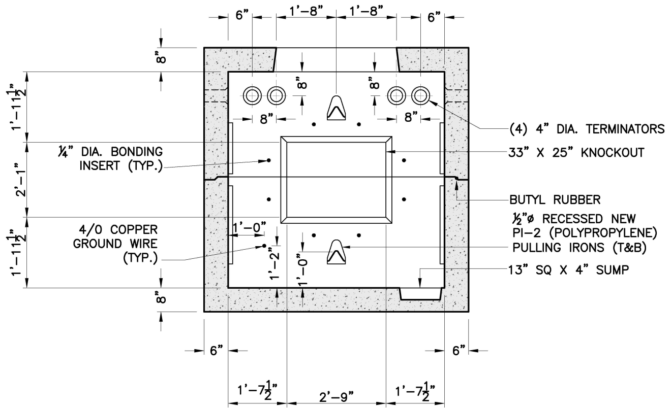
SECTION B-B OPPOSITE WALLS ARE MIRROR IMAGES.
