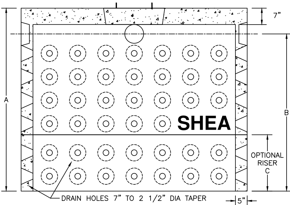
SECTION VIEW
