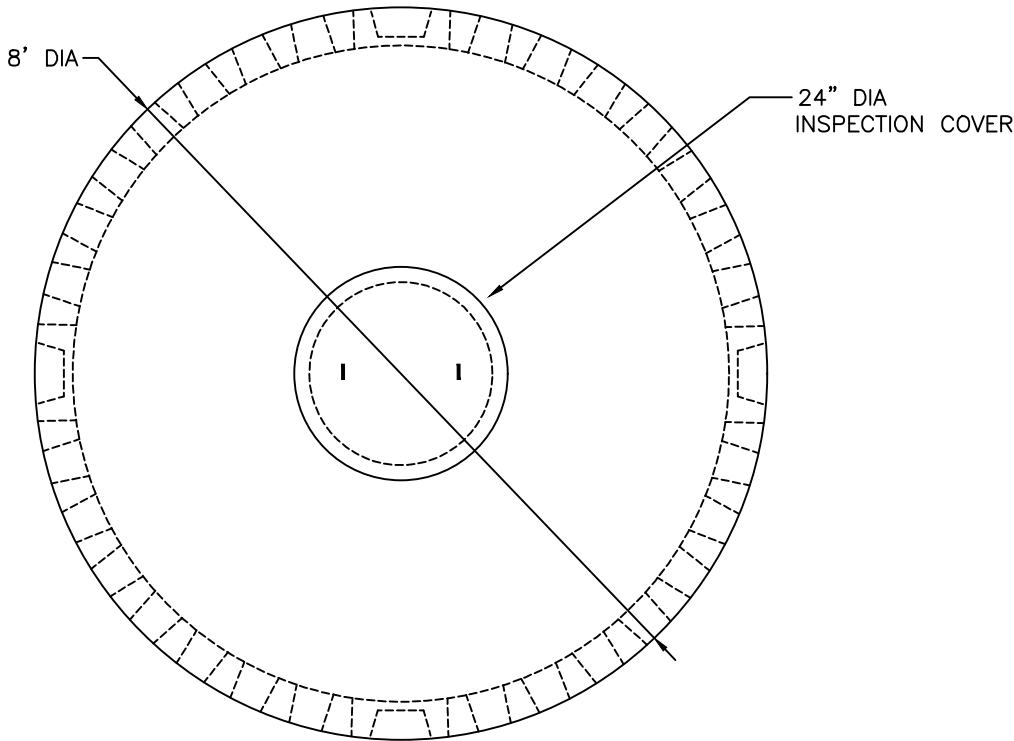
PLAN VIEW
