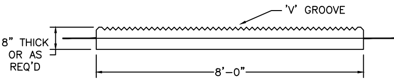
END VIEW
