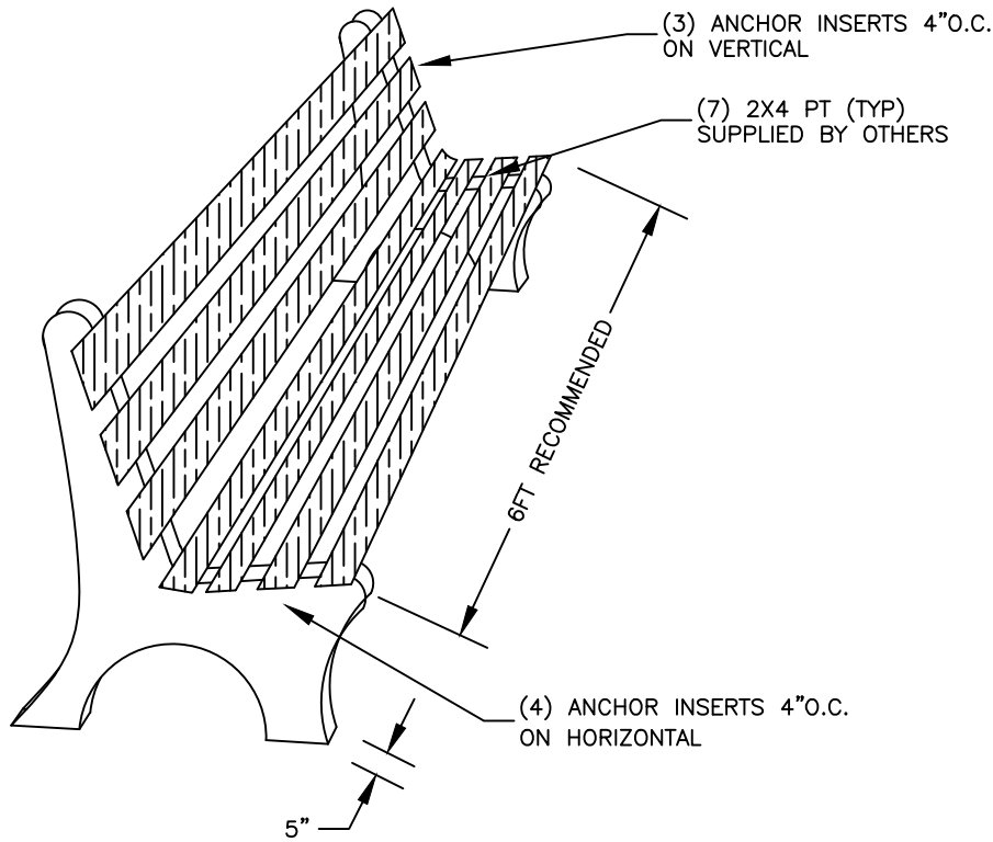
ISO VIEW
