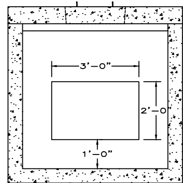
SECTION B-B VIEW
