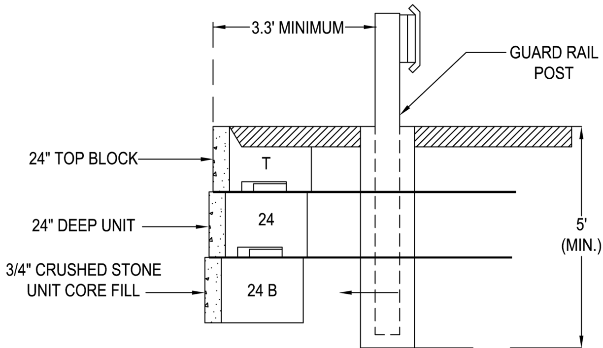
GUARD RAIL DETAIL NOT TO SCALE
