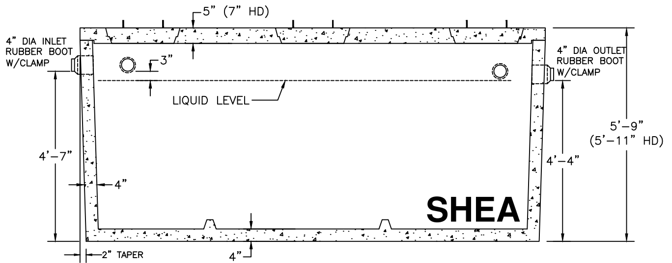
SECTION VIEW
