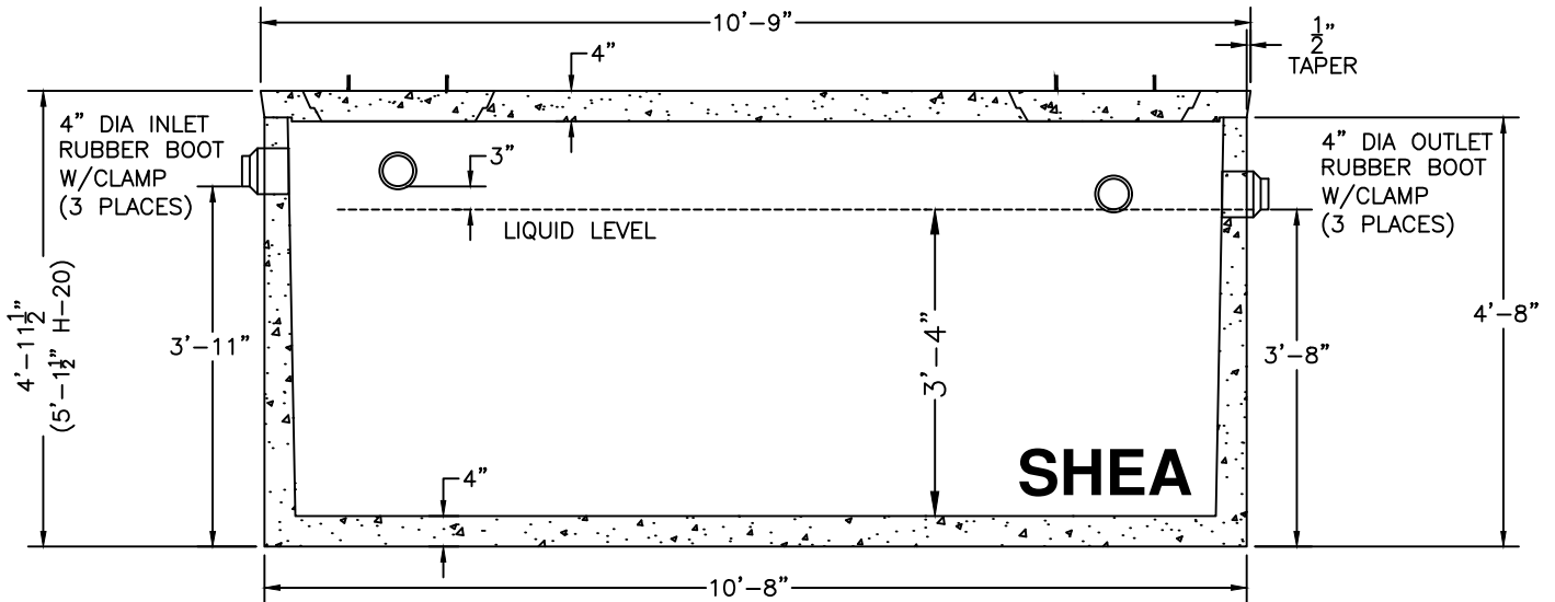
SECTION VIEW
