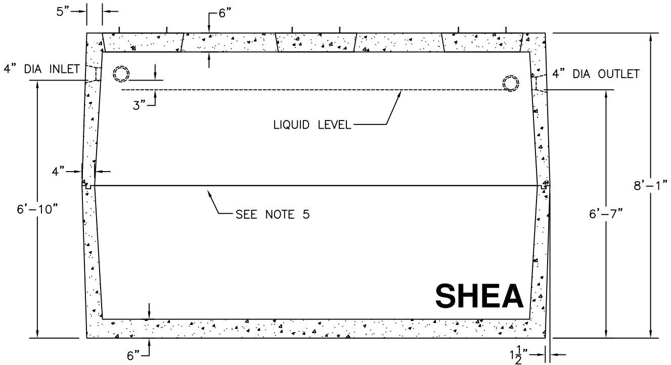
SECTION VIEW
