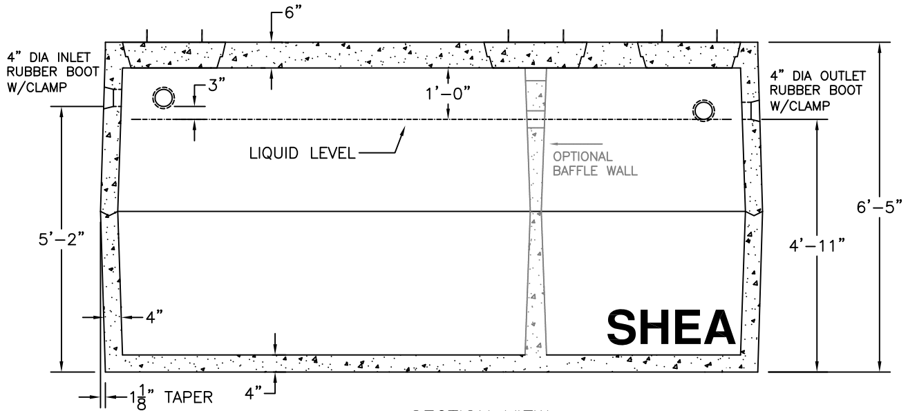
SECTION VIEW
