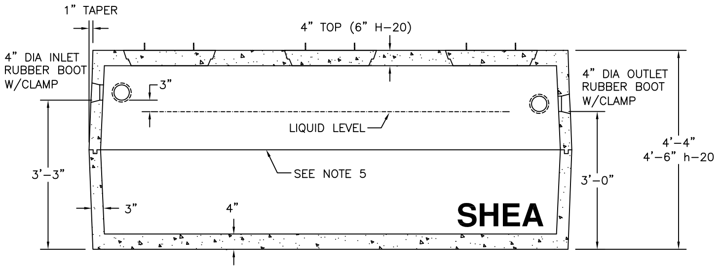
SECTION VIEW
