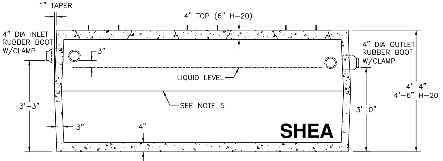
SECTION VIEW
