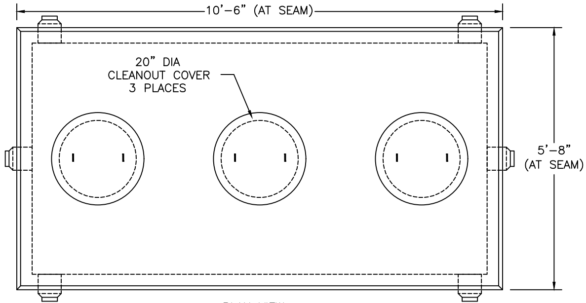
PLAN VIEW
