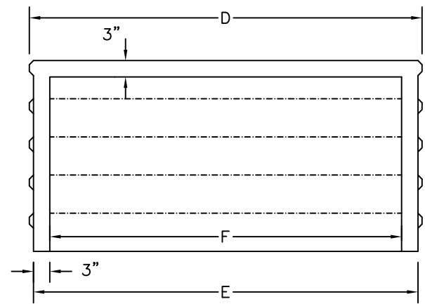
END VIEW
