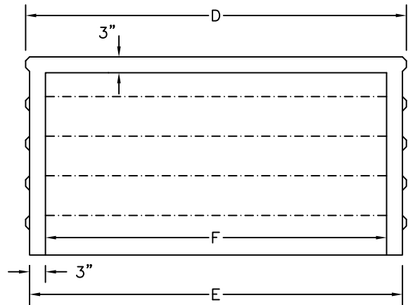
END VIEW
