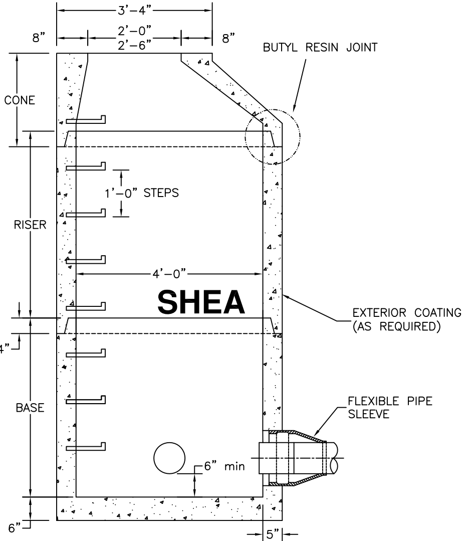
SECTION VIEW
