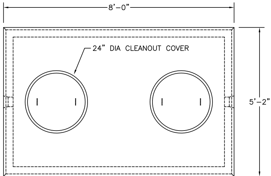
PLAN VIEW
