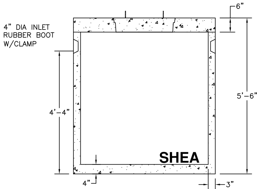
SECTION VIEW
