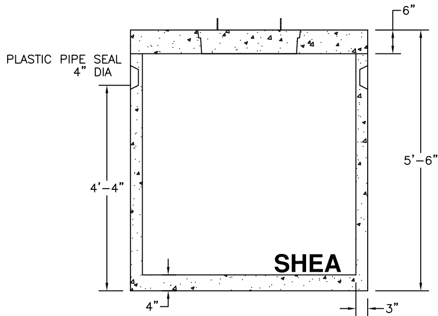
SECTION VIEW
