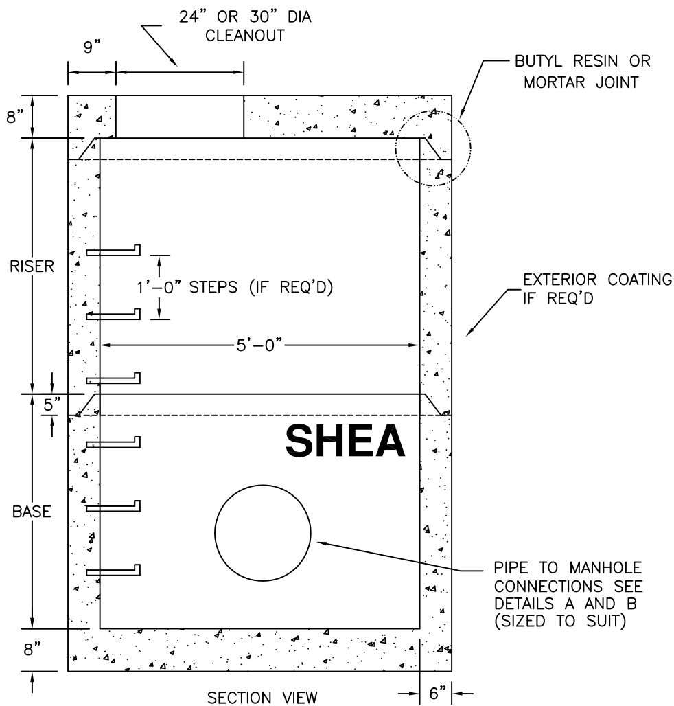
RISER SECTION
