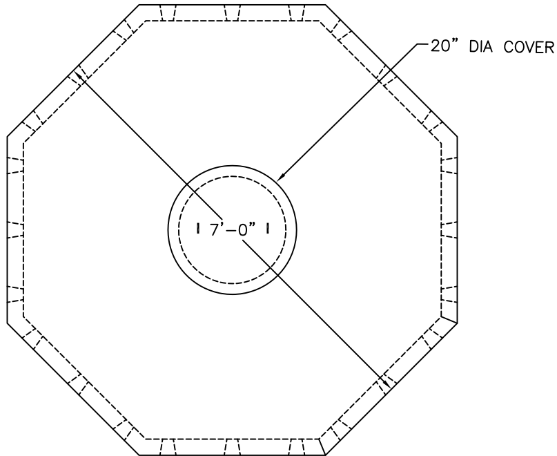
PLAN VIEW
