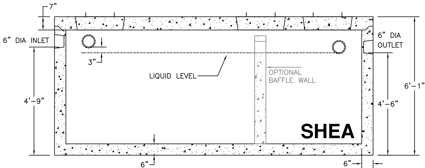
SECTION VIEW
