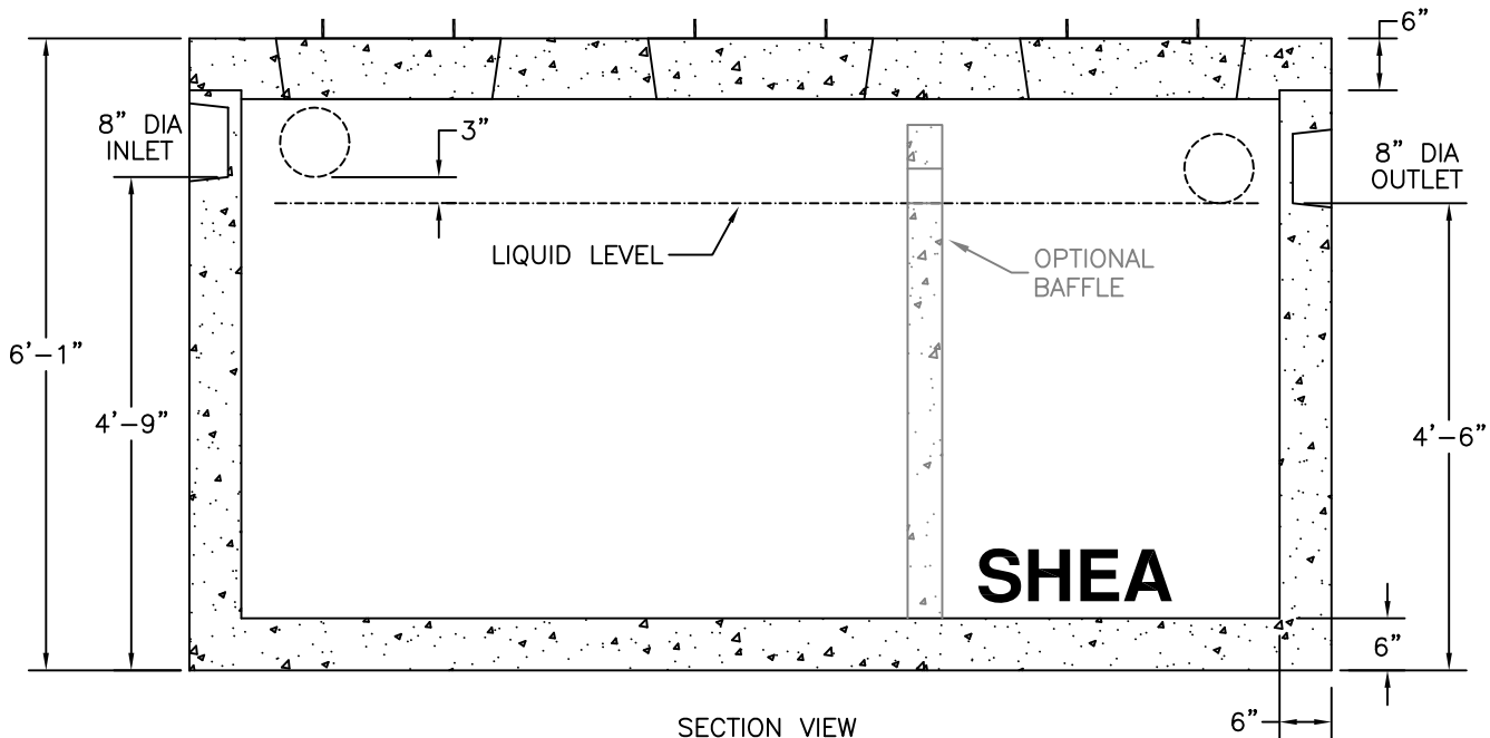
SECTION VIEW
