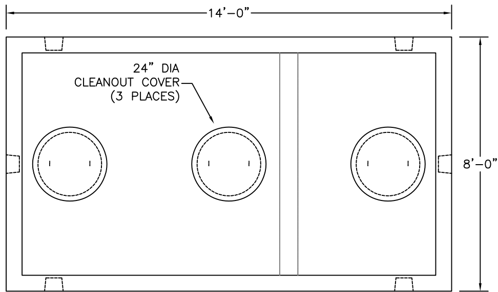
PLAN VIEW
