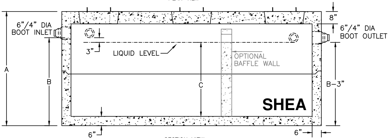
SECTION VIEW
