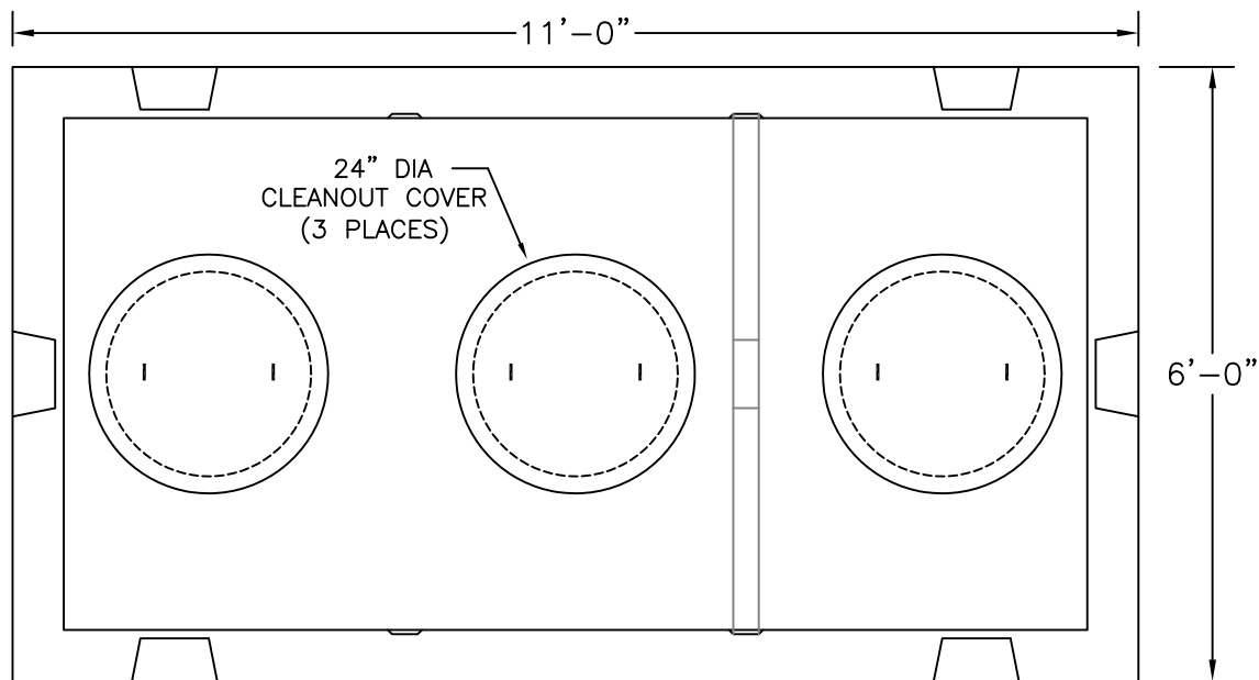
PLAN VIEW
