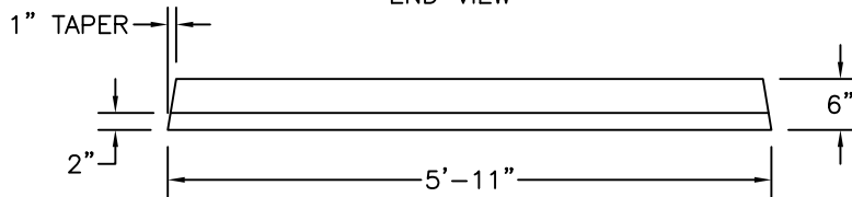
SIDE VIEW
