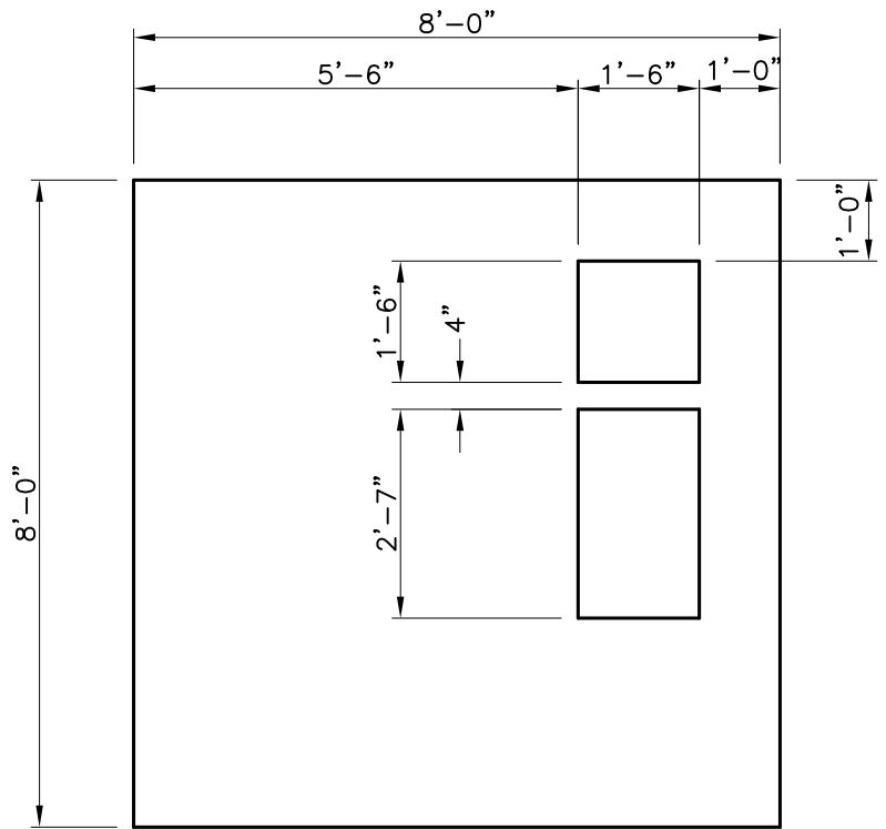
TRANSFORMER PAD - PLAN
