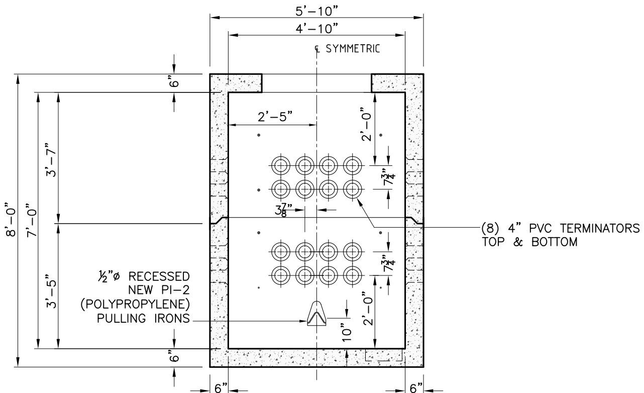
SECTION B-B OPPOSITE WALLS ARE MIRROR IMAGES.
