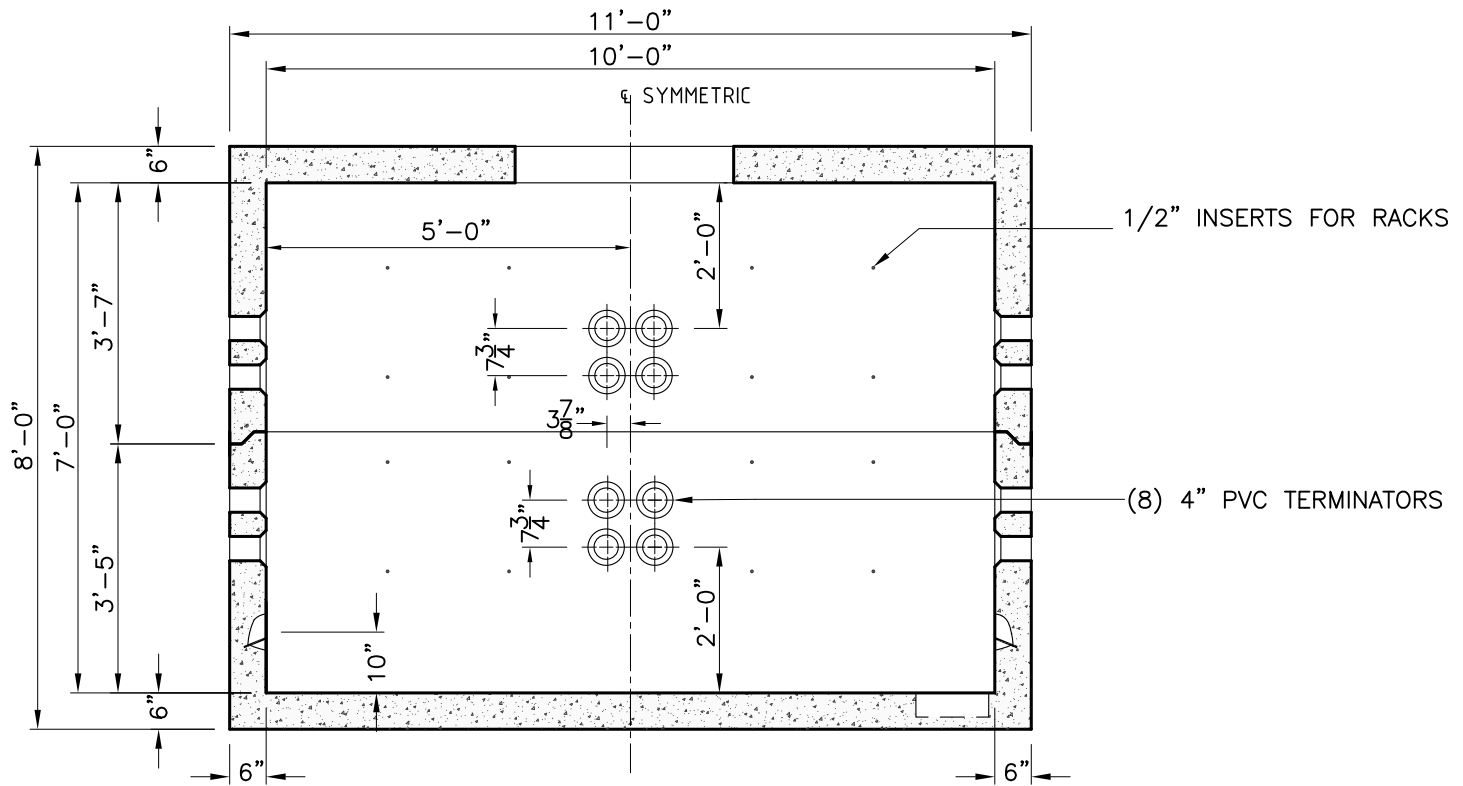
SECTION A-A OPPOSITE WALLS ARE MIRROR IMAGES.
