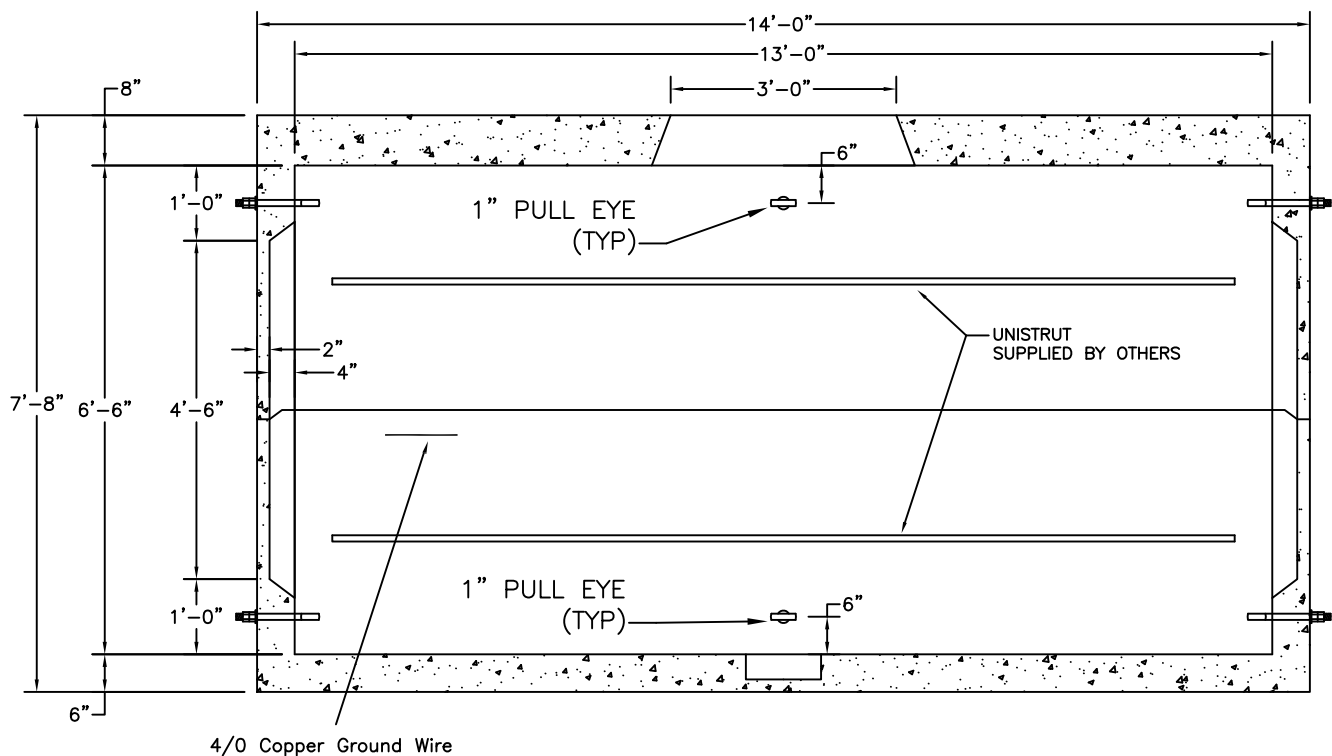
SECTION AA
