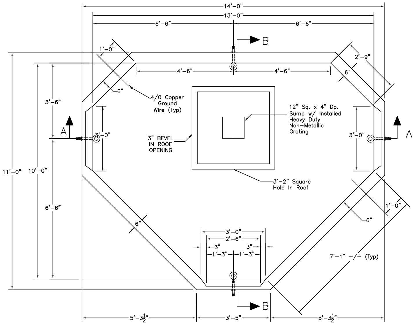
PLAN VIEW
