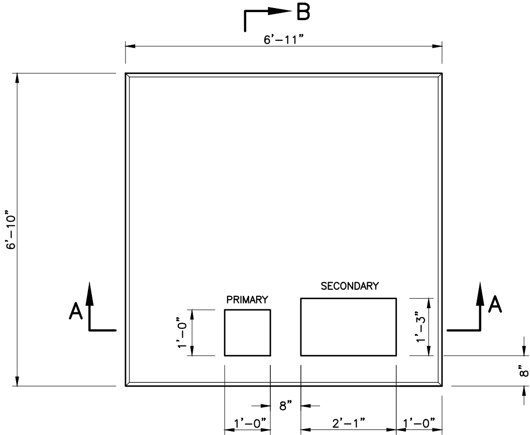
PLAN
