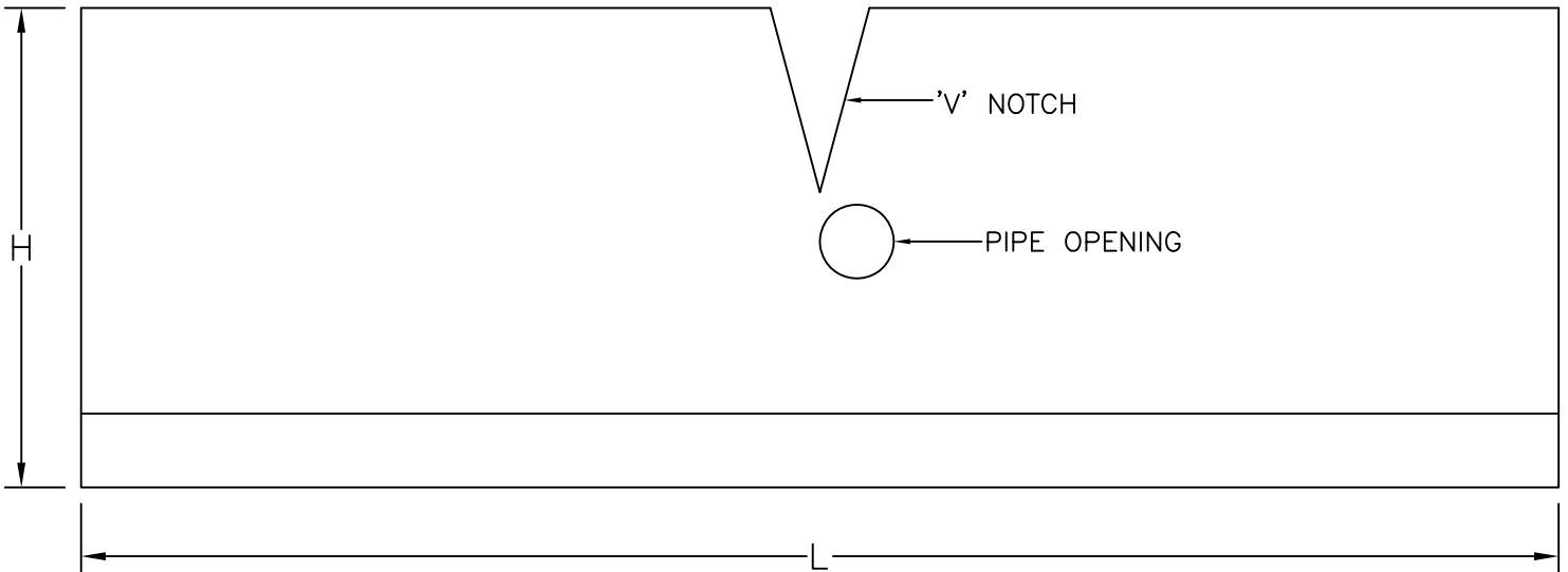
FRONT VIEW
