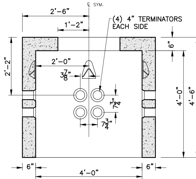
SECTION A-A OPEN BOTTOM
