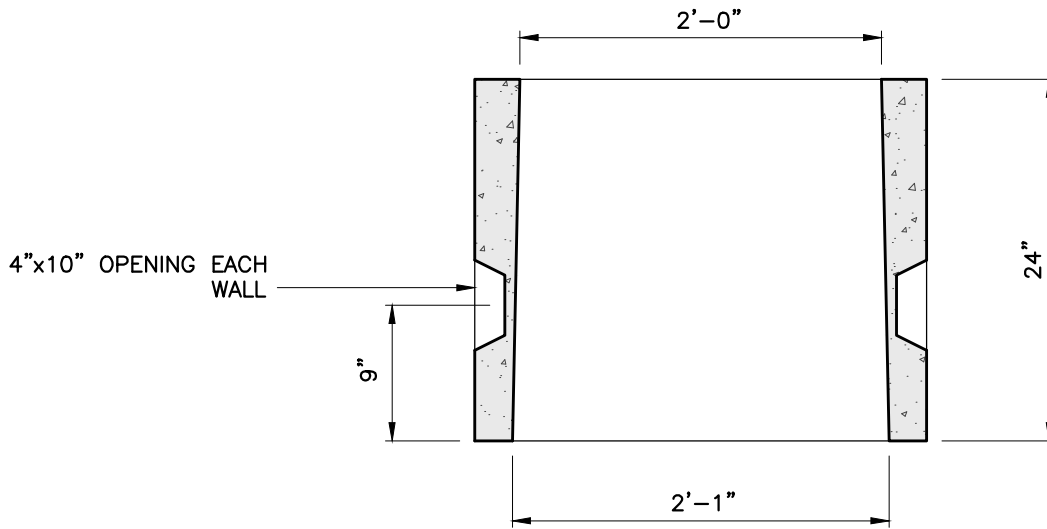
SECTION A-A OPPOSITE/ADJACENT WALLS SIMILAR
