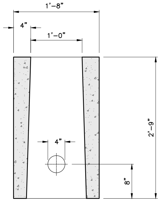
SECTION B-B
