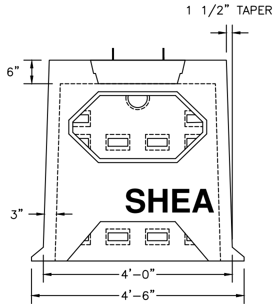
BACK VIEW
