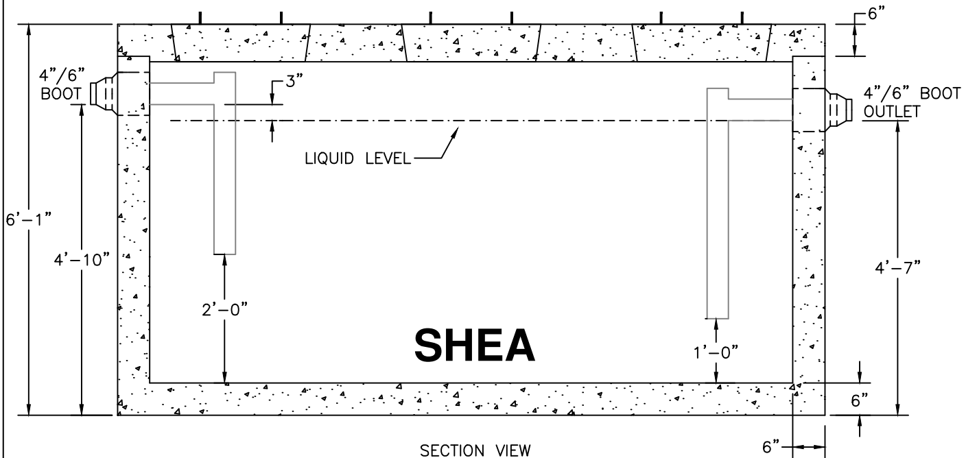
SECTION VIEW
