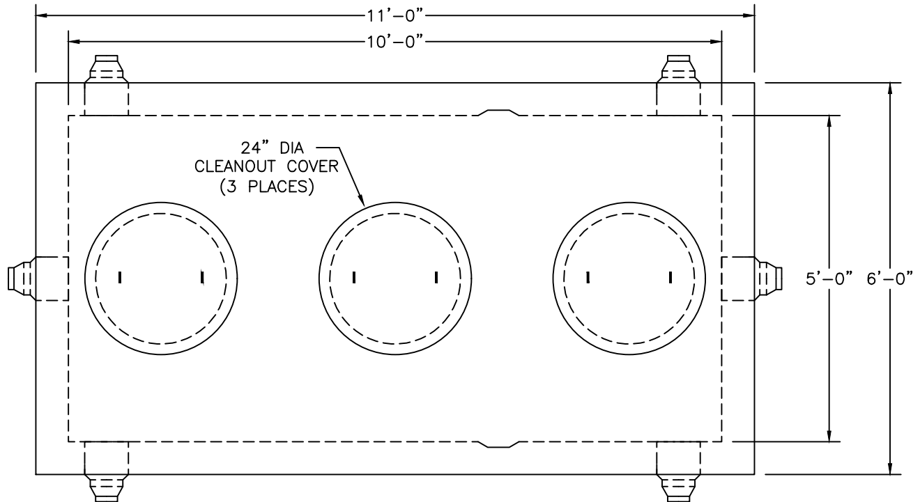
PLAN VIEW
