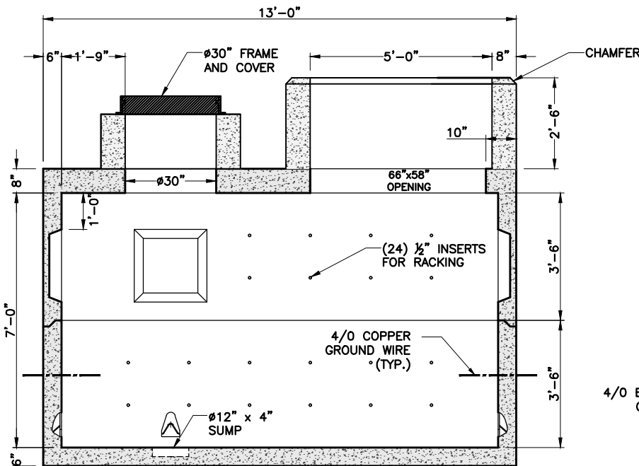
SECTION A-A OPPOSITE WALL SIMILAR
