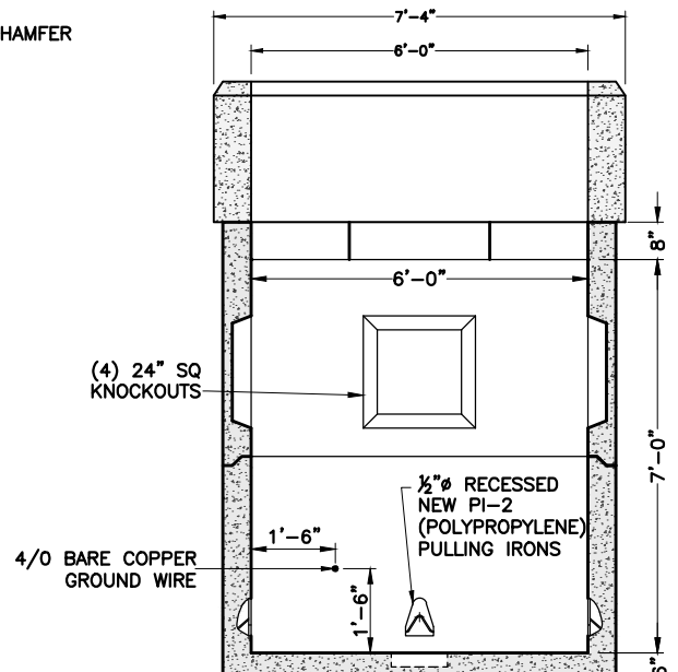
SECTION B-B OPPOSITE WALL SIMILAR
