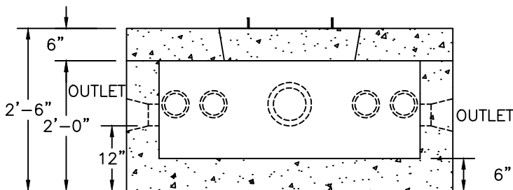
INLET VIEW
